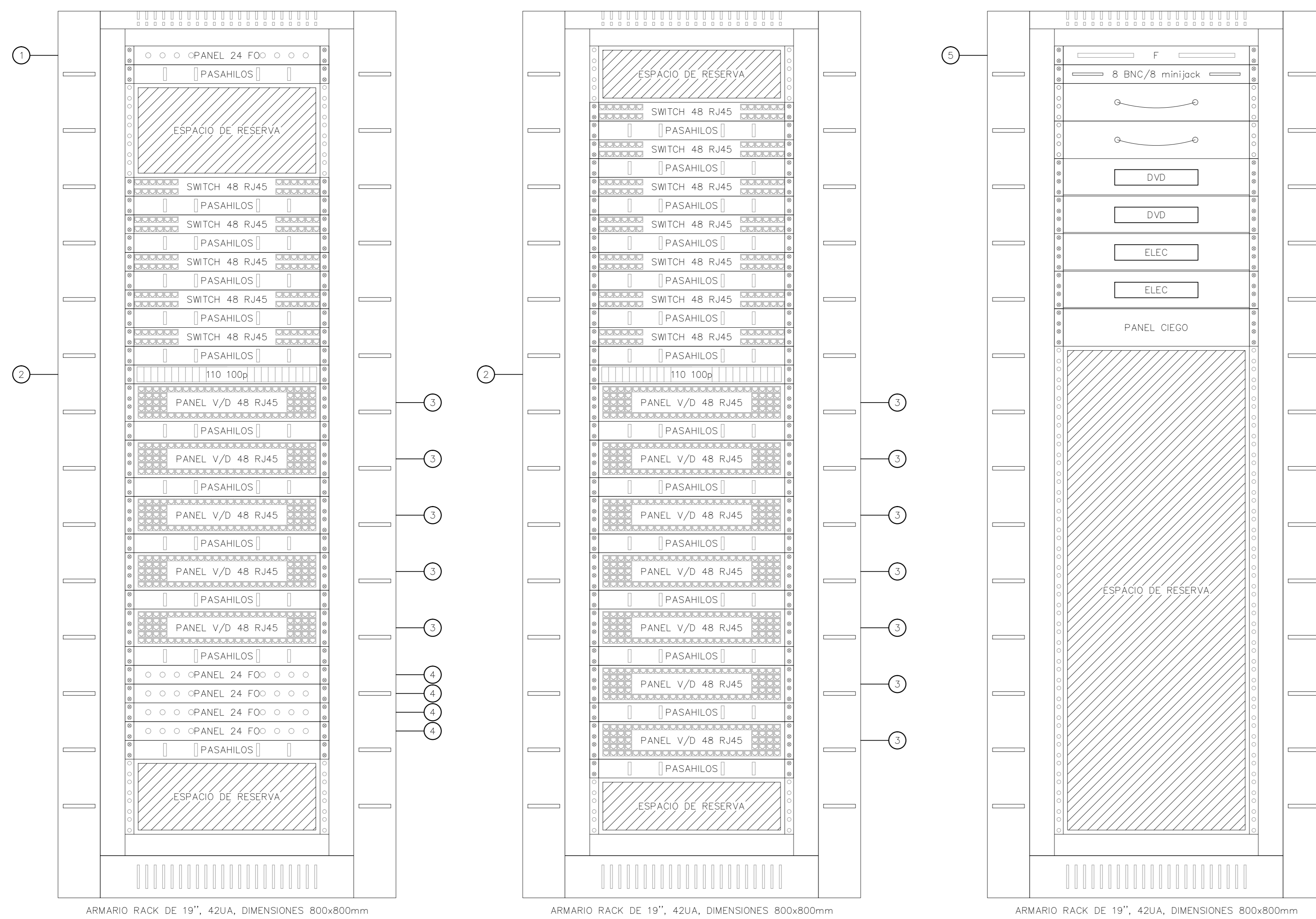
ARMARIO RACK DE 19", 42UA, DIMENSIONES 800x800mm
