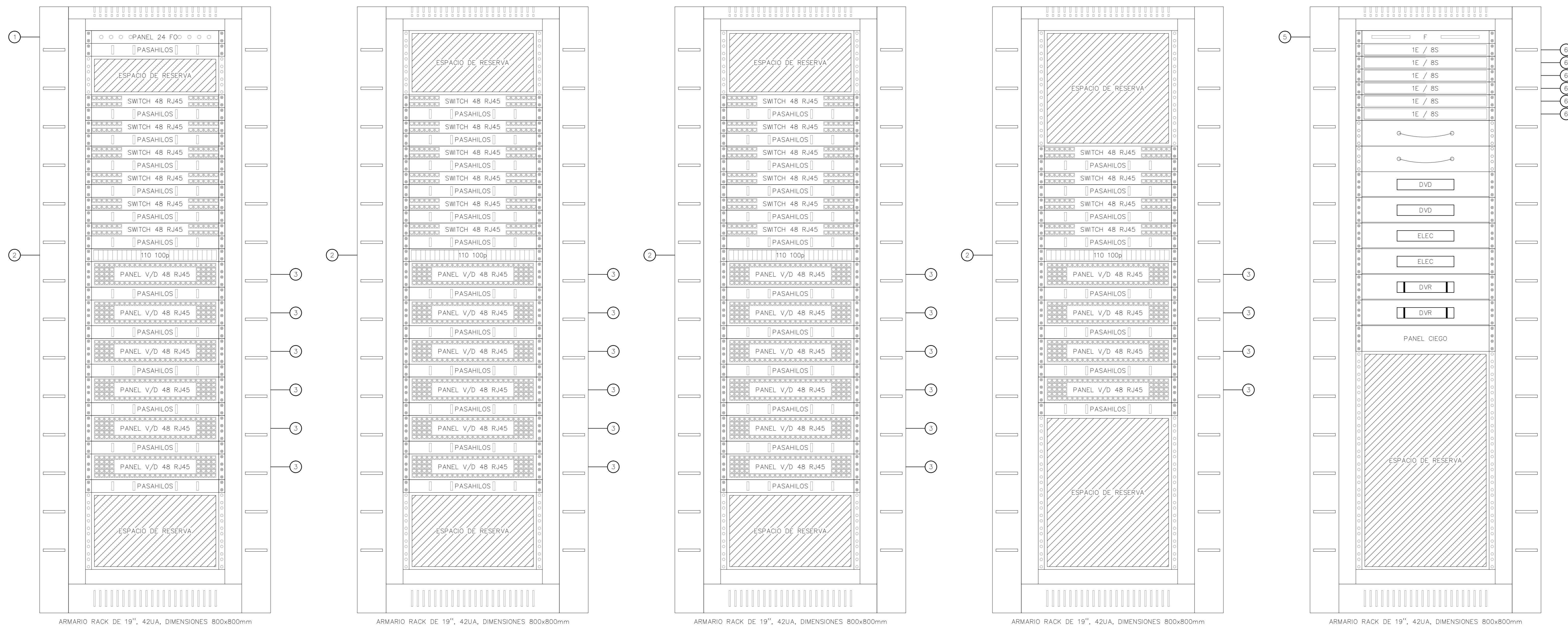
ARMARIO RACK DE 19", 42UA, DIMENSIONES 800x800mm
